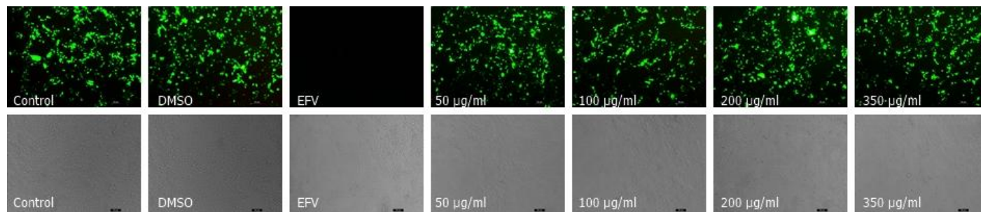
FIG- Anti HIV-1 activity of Swertia bimaculata Chloroform extract: In a 96 well plate HIV-1 infected Huh 7.5 cells were grown in presence of different concentrations of Swertia bimaculata Chloroform extract. After 48h and 72h expression of GFP reporter was evaluated by fluorescent microscopy. As seen in the images above there is no distinct reduction in GFP positive foci in cells treated with increasing concentration of Chloroform extract, indicating Swertia bimaculata Chloroform extract have no anti HIV-1 activity. Upper panel shows the fluorescence microscopy and the lower plane shows bright filed microscopy.
