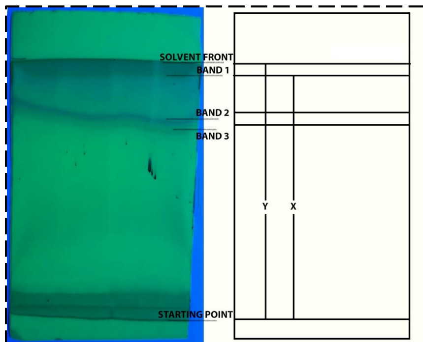
Thin Layer chromatography to identify components of E3M7 (Ethyl Acetate 30%+ Methanol 70% - Methanolic Extract of Ocimum gratissimum) showing three bands.
